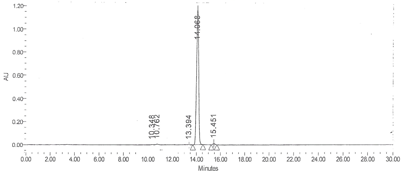
Auto-Scaled Chromatogram
